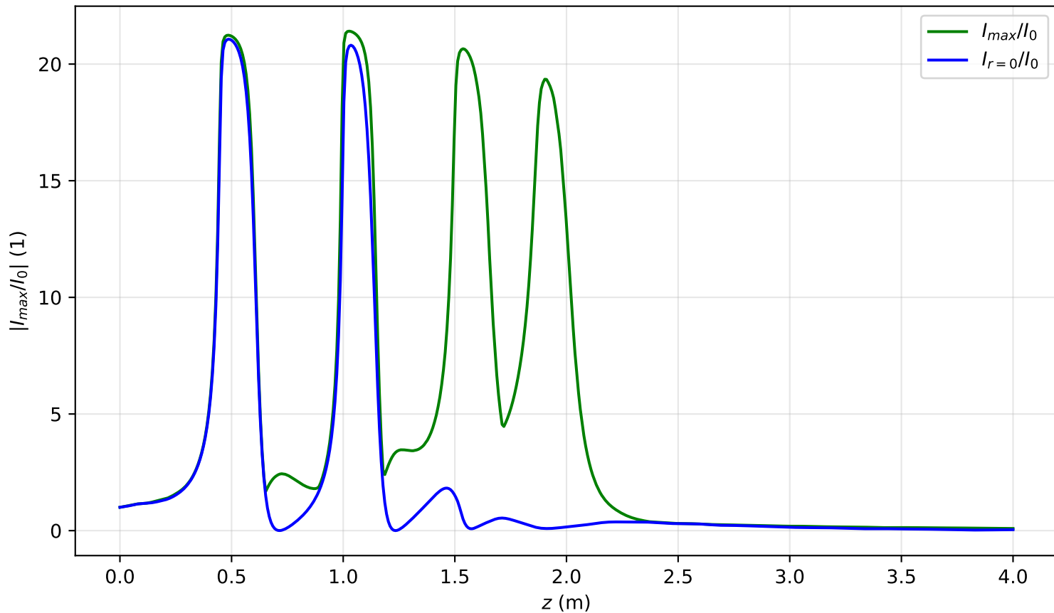
I_{max}(x = 0, y = 0, z)/I_0 , P_{in}=5.2P_{cr} , noisy input, artificial time
